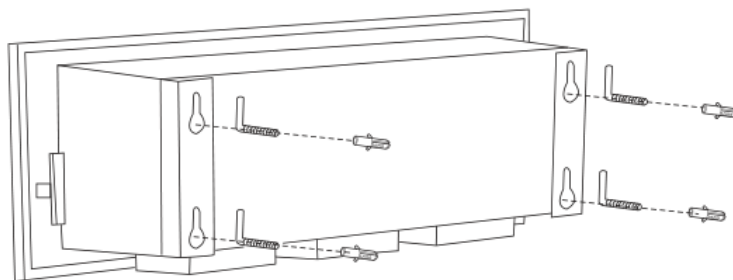
Wall mounted (with hooks)
