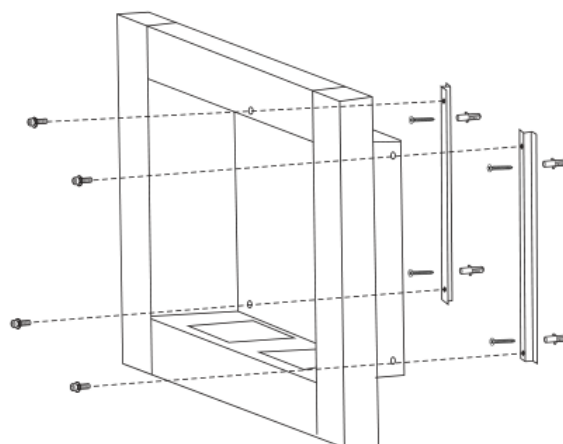
Wall mounted (with brackets)
